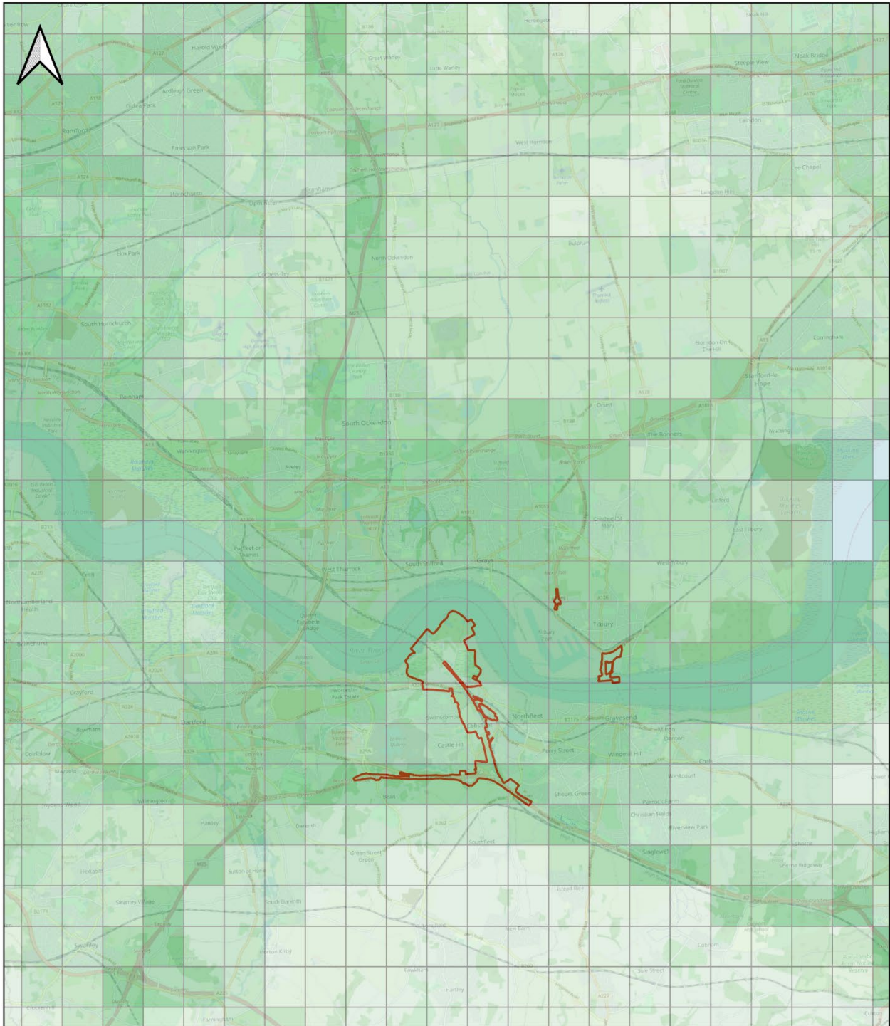
Figure 16.13 NOx Background Concentrations
